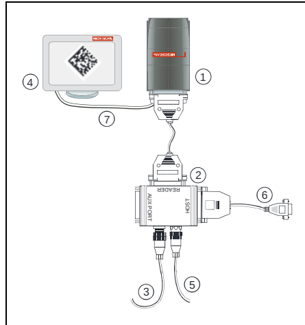
Hardware Configuration
