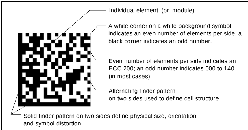
Data Matrix Symbol Comparison
