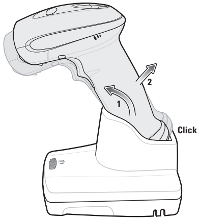
Figure 1-13 Removing the Digital Scanner in the Cradle
