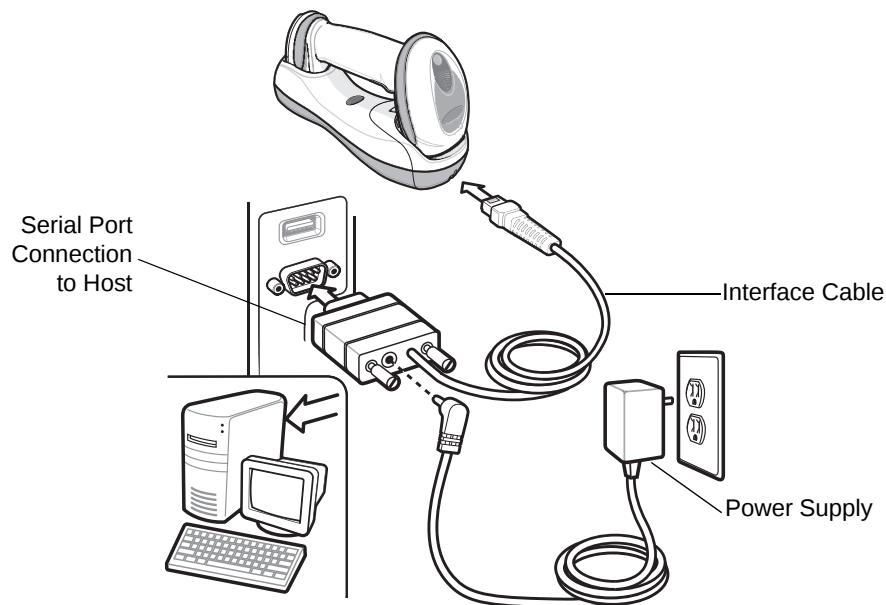
Figure 8-1 RS-232 Direct Connection
