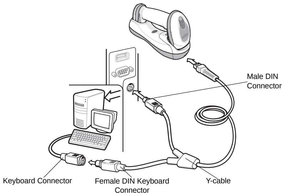
Figure 9-1 Keyboard Wedge Connection with Y-cable
