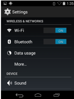
Figure 3-31 Settings Screen
