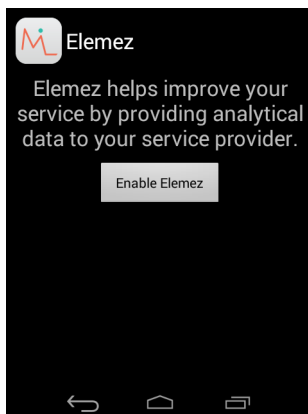
Figure 3-28 Elemez Application
