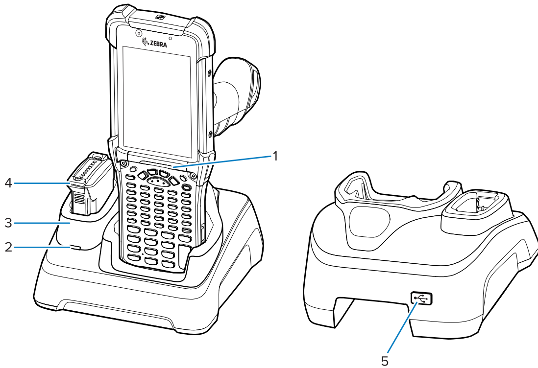
Figure 24 1-Slot USB Charge Cradle with Spare Battery Charger
