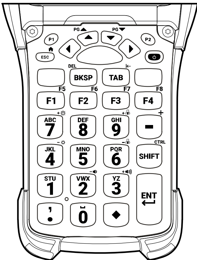
Figure 57 29-Keys Shifted Alpha Keypad
