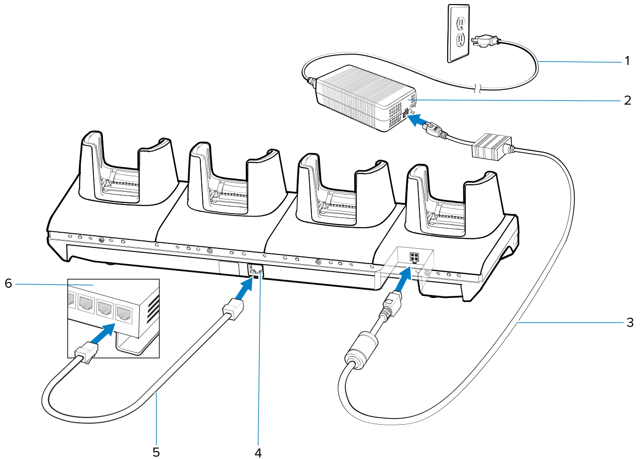
Figure 31 4-Slot Ethernet ShareCradle Setup
