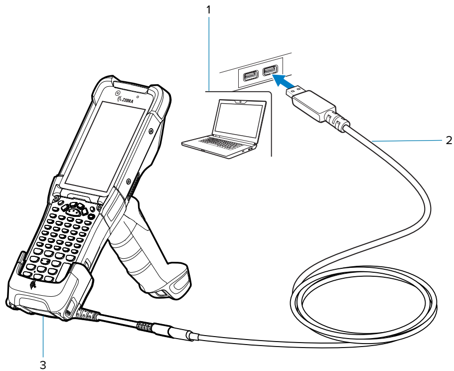
Figure 42 Connecting USB Charge/Com Snap-on Cup to Host Computer
