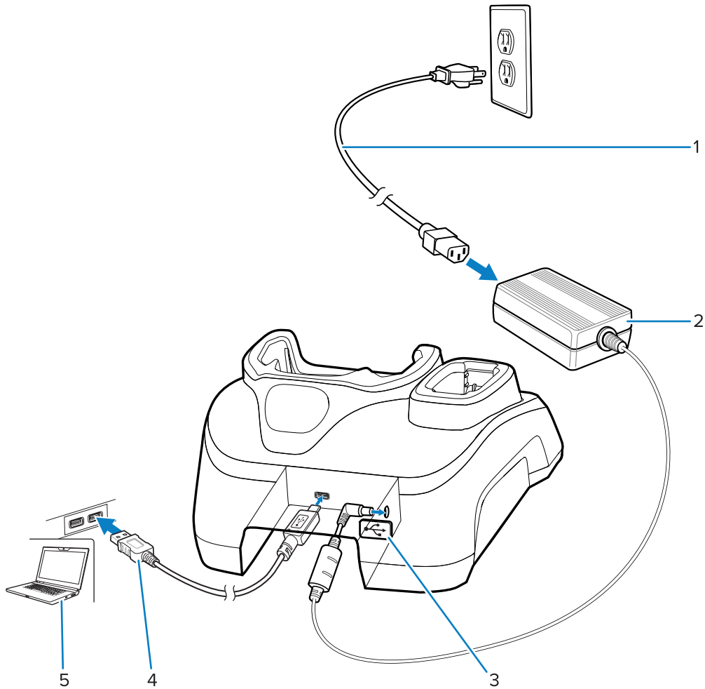
Figure 25 1-Slot USB Charge Cradle with Spare Battery Charger Setup
