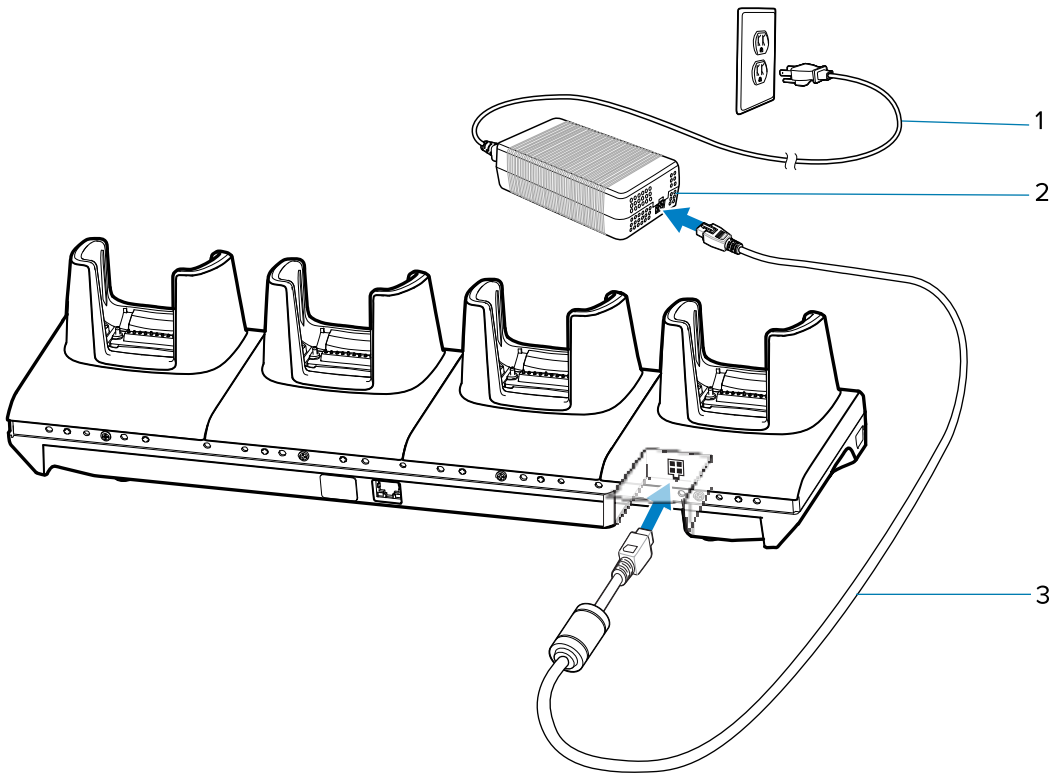
Figure 28 4-Slot Charge Only ShareCradle Setup
