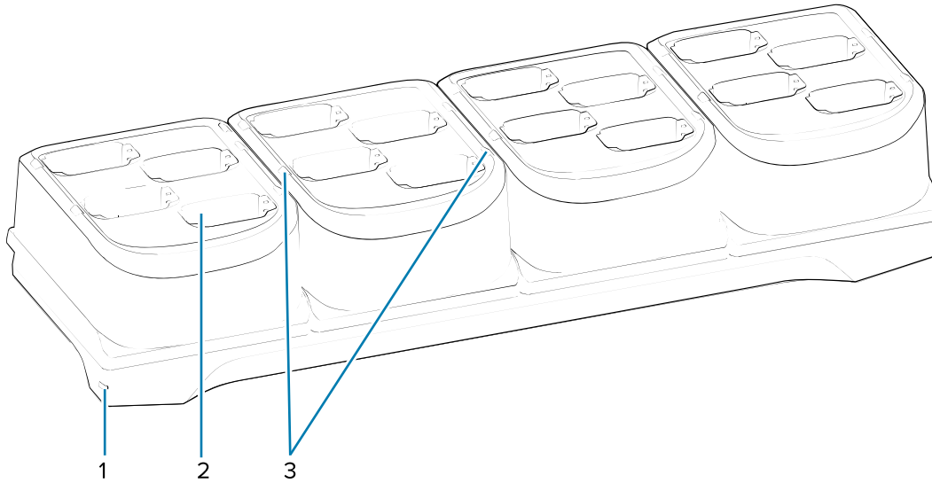
Figure 37 16-Slot Spare Battery Charger
