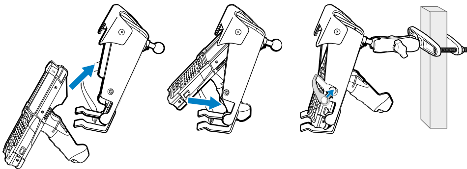
Figure 47 Insert Device into Forklift Mount Holder, Rotate and Snap (Option 2)
