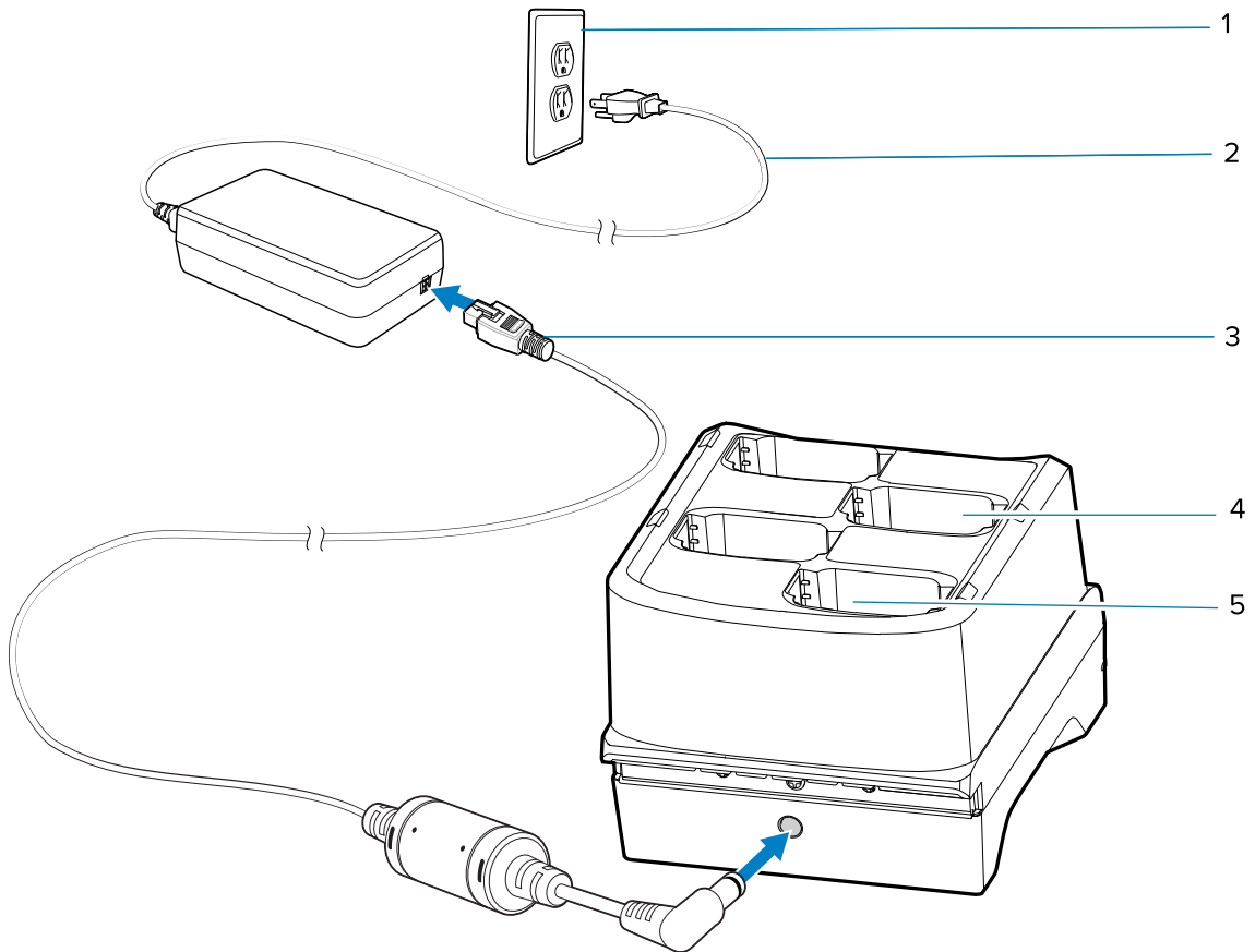
Figure 35 4-Slot Spare Battery Charger Setup
