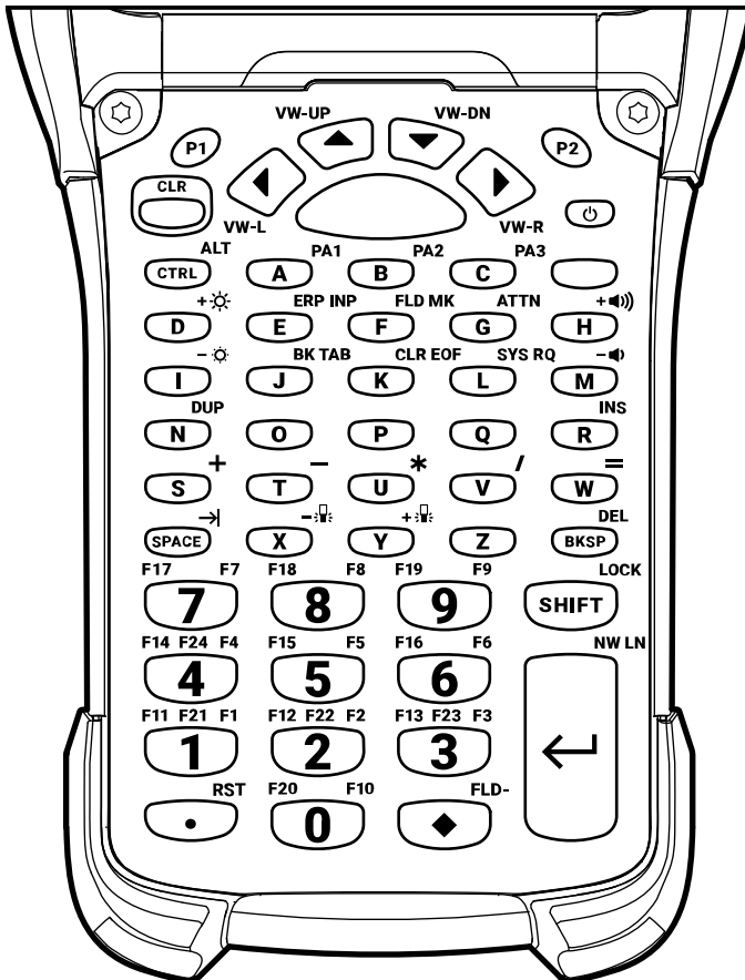
Figure 53 53-Keys IBM-3270 Emulator Keypad
