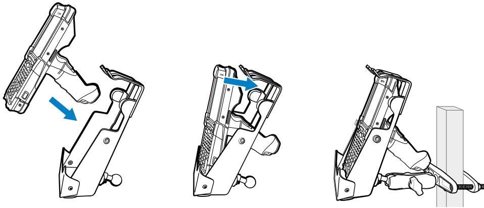
Figure 47 Insert Device into Forklift Mount Holder, Rotate and Snap (Option 2)
