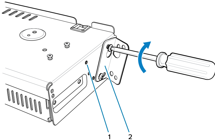
Figure 49 Flange 25° Position (4-Slot Battery Chargers)
