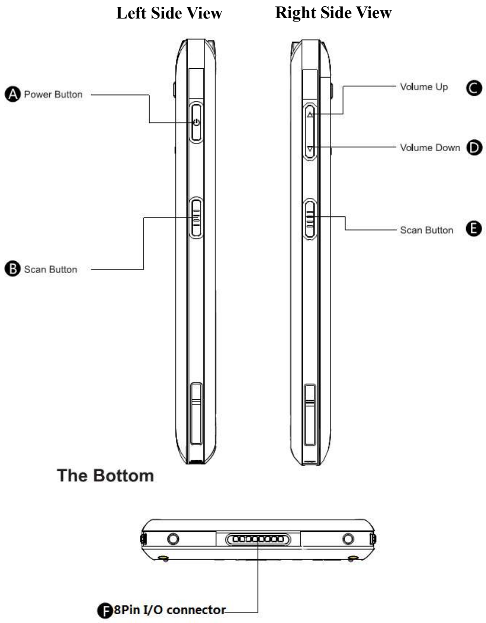
Side and bottom views of the EDA70-X
