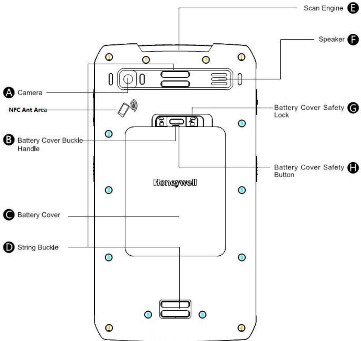
Back view of the EDA70-X
