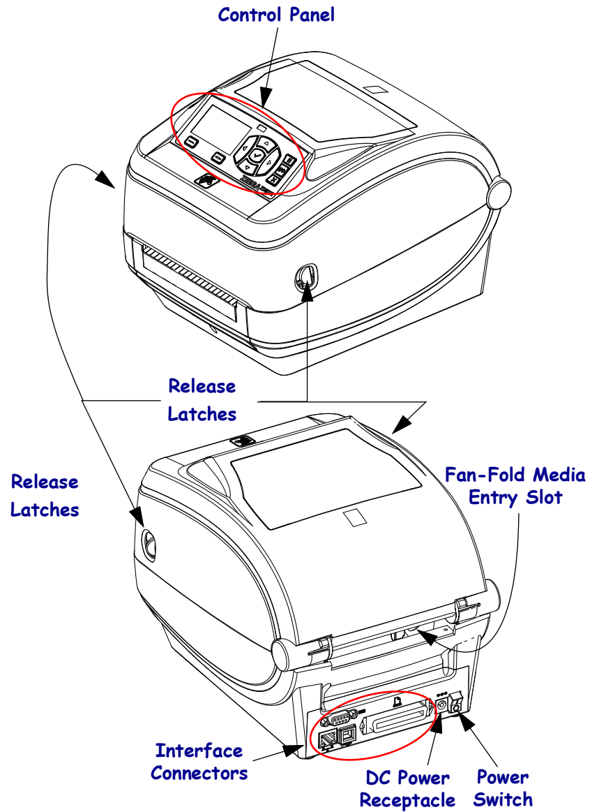
Figure 1 • Printer Features
